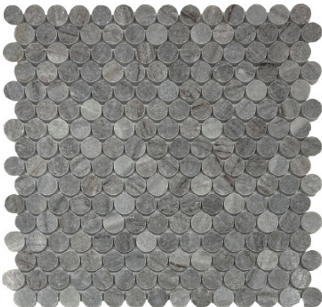
Penny Round Polished / Honed 11.25" x 11.25", 3/8" thick BVPPR/BVHPR
